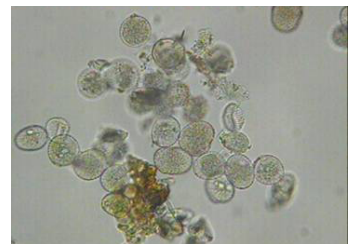
Urediniospores
