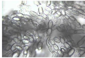
Conidia
