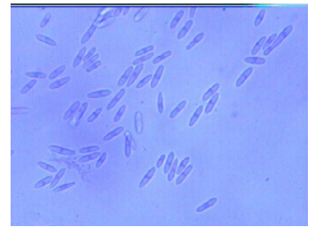
Conidia
